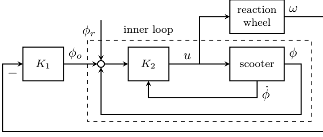
Fig. 2. Control structure.
