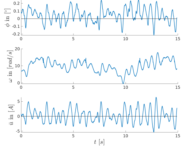
Fig. 3. Measurements of the tilt angle \phi , the angular velocity of the reaction wheel \omega , and input \bar{u} of the balancing e-scooter. The signals are filtered with a first order filter.
