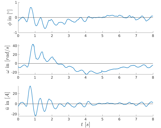
Fig. 4. Measurements of the tilt angle \phi , the angular velocity of the reaction wheel \omega , and input \bar{u} of the e-scooter when being pushed at the handle bar at t = 0.5\text{s} . The signals are filtered with a first order filter.
